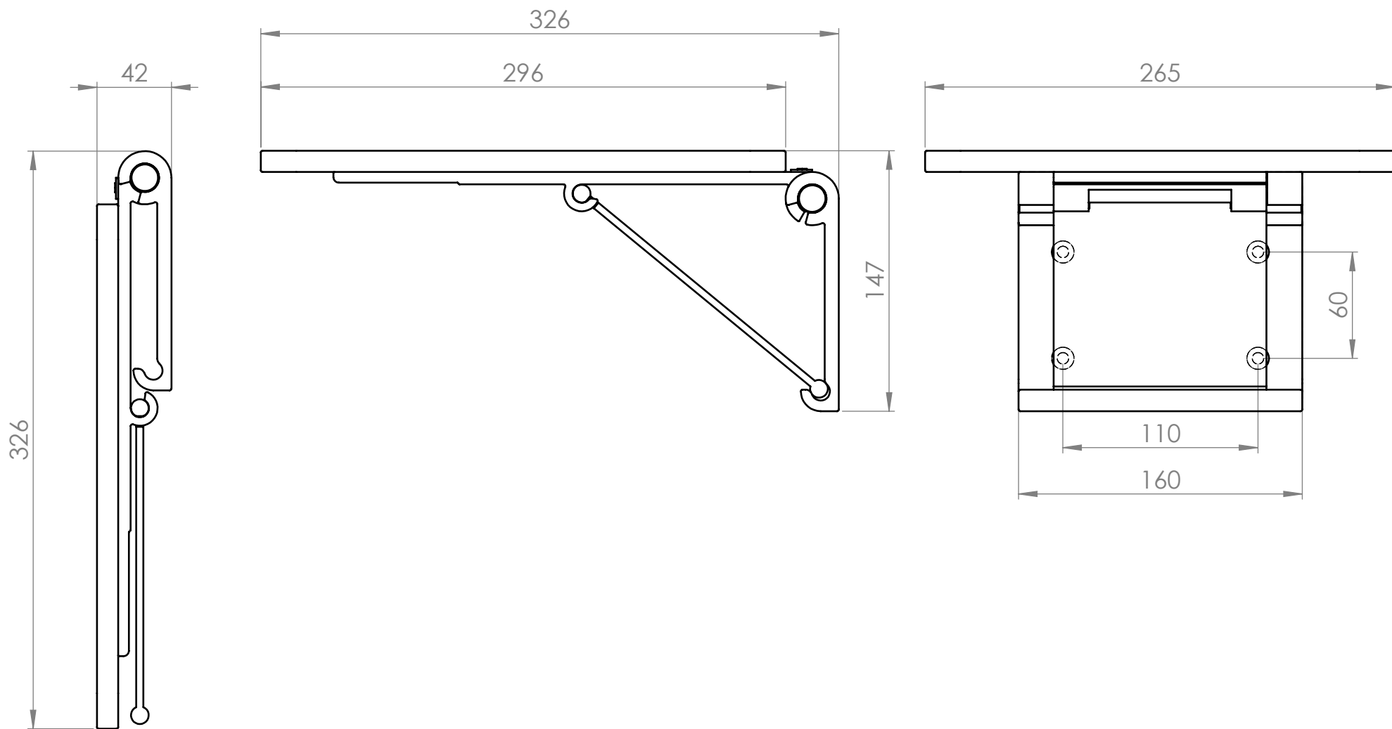
Compact shower seat LI2201.2013-02
